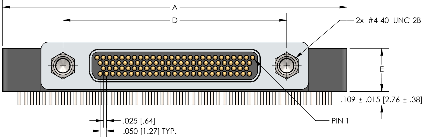
FRONT VIEW - PLUG (PINS)
